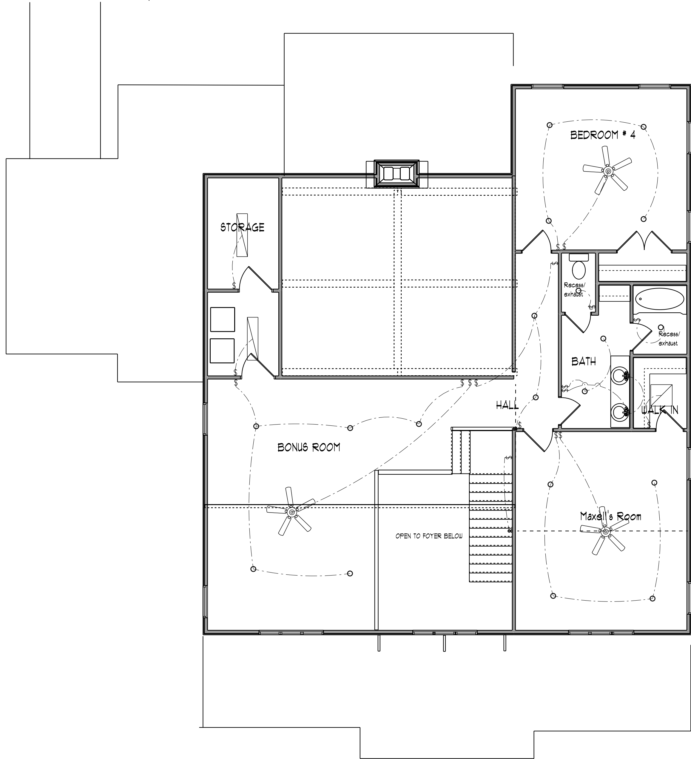
SECOND FLOOR FINAL - ELECTRICAL SCALE: 3/16" = 1'-0"
