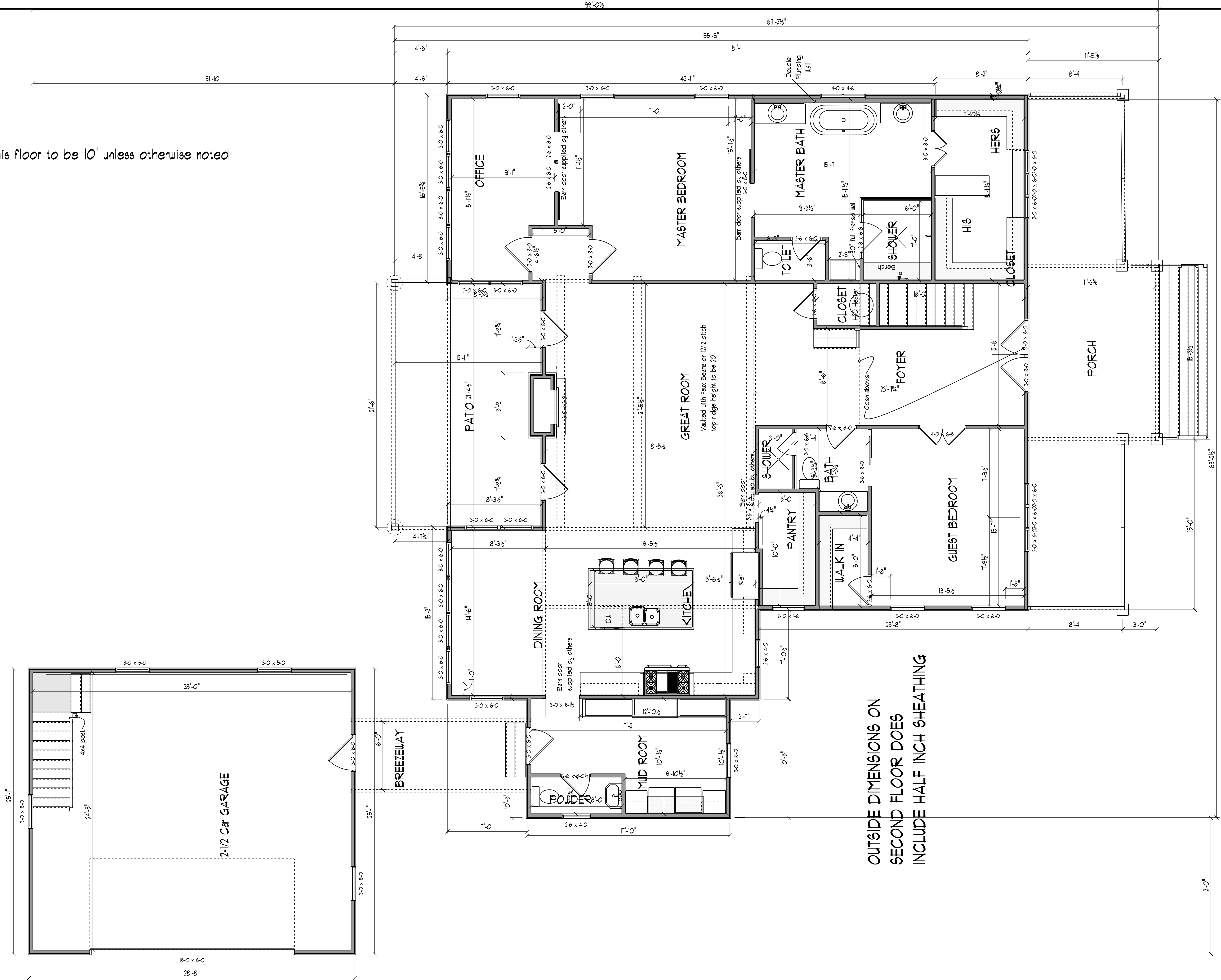
MAIN FLOOR FINAL SCALE: 1/4" = 1'-0"
