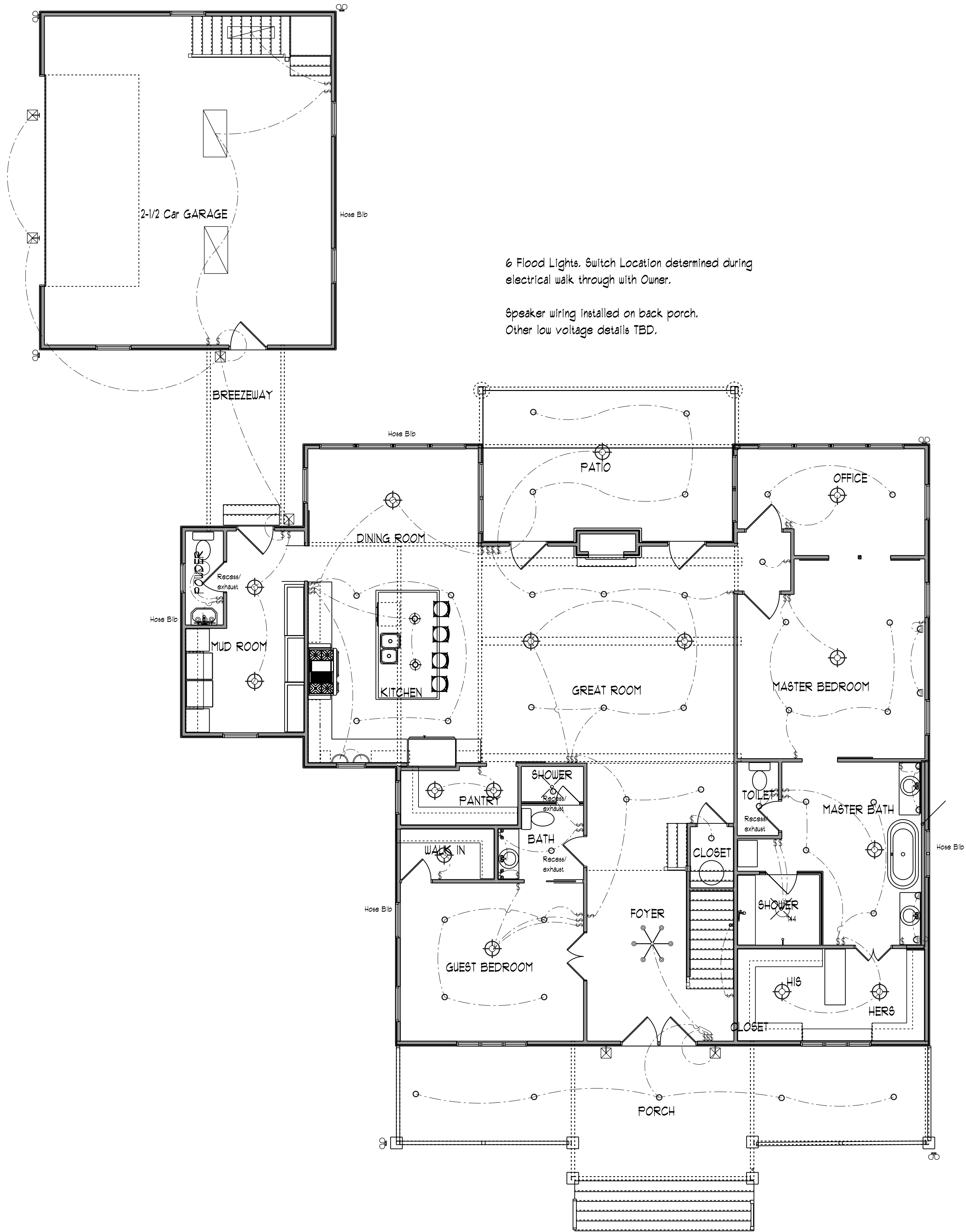
MAIN FLOOR FINAL - ELECTRICAL SCALE: 3/16" = 1'-0"
